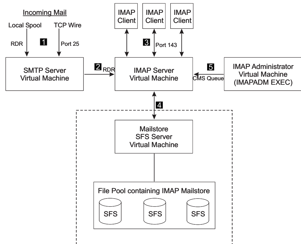
Figure 78. IMAP Client and Server Environment
